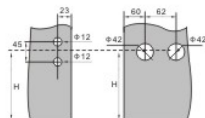
Glass to glass lock with stainless steel cover
