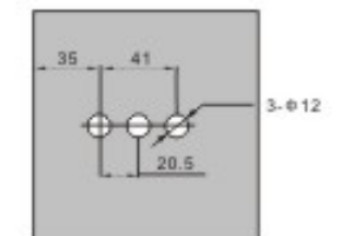
Glass to wall lock with stainless steel cover
