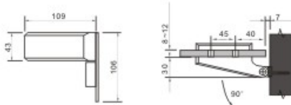
Bifold hinge
