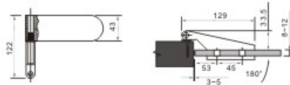
Bifold hinge
