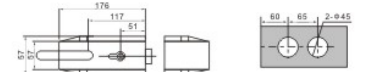
Glass to wall lock
